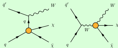
Mono-W + \cancel{E}_T
